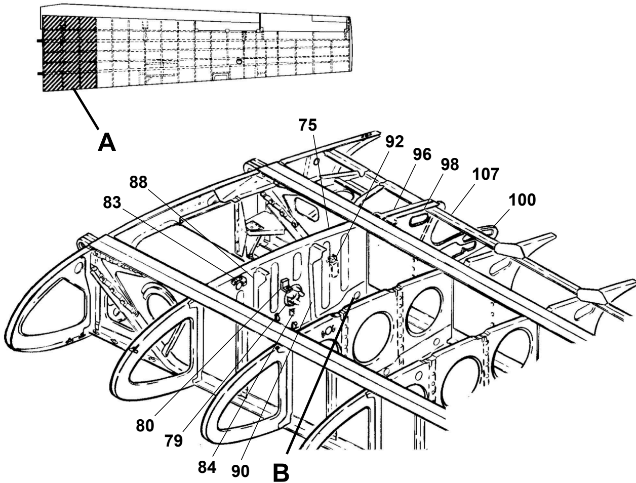
DETAIL A
