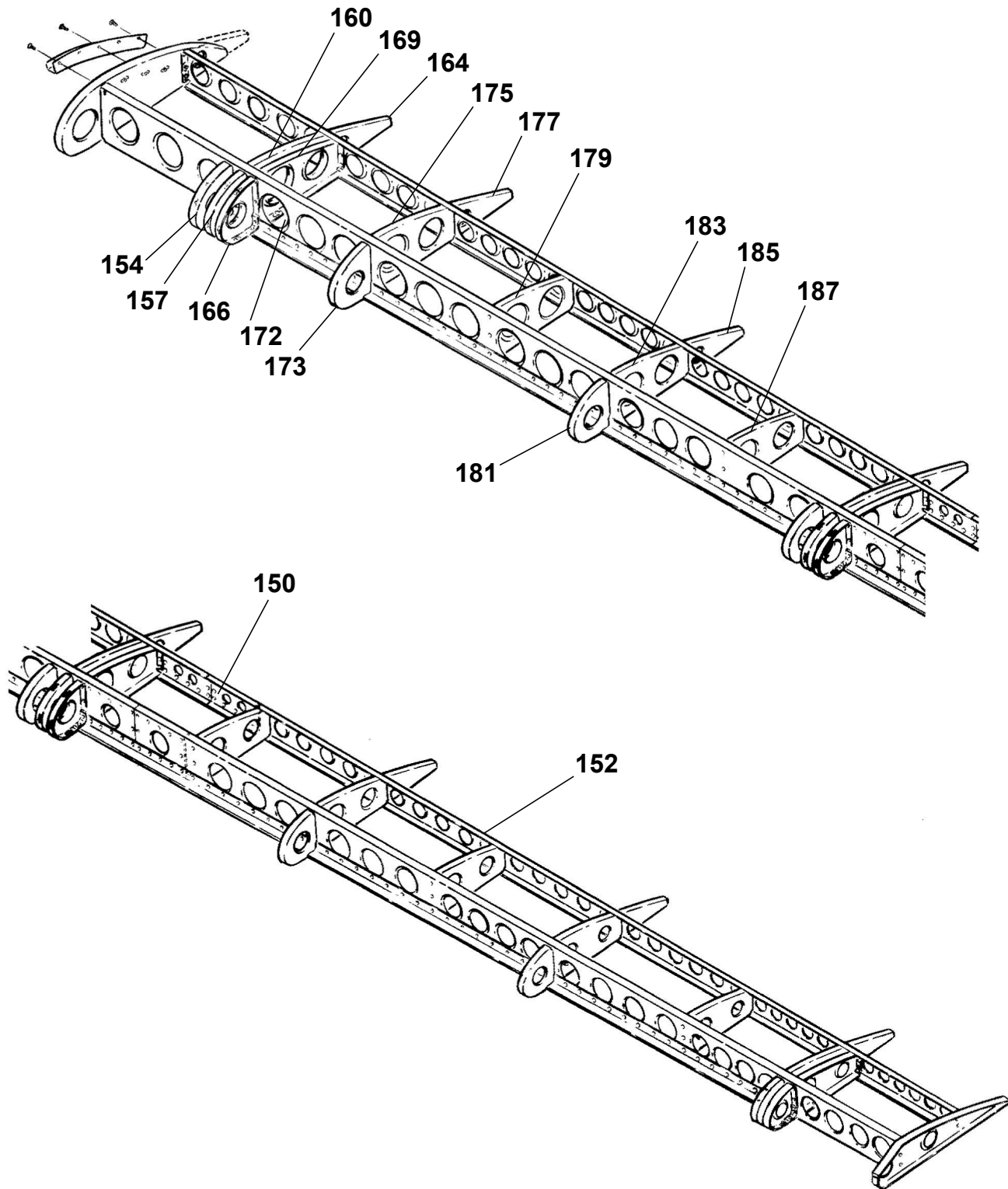
FLAP ASSEMBLY - STRUCTURE Figure 02. (Sheet 3)
