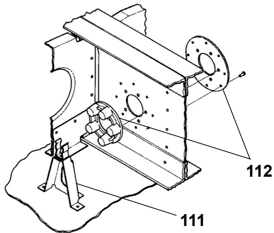
WING STRUCTURE COMPONENTS - FUEL BAY CENTER OUTBOARD Figure 03. (Sheet 2)
