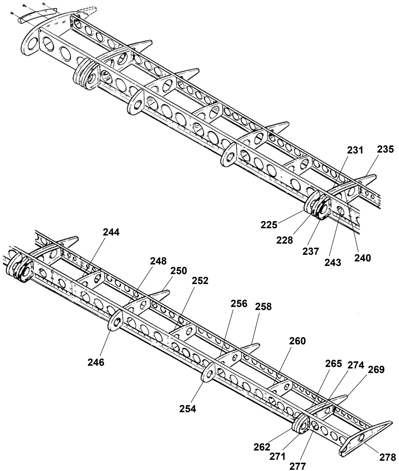
FLAP ASSEMBLY - STRUCTURE Figure 02. (Sheet 4)
