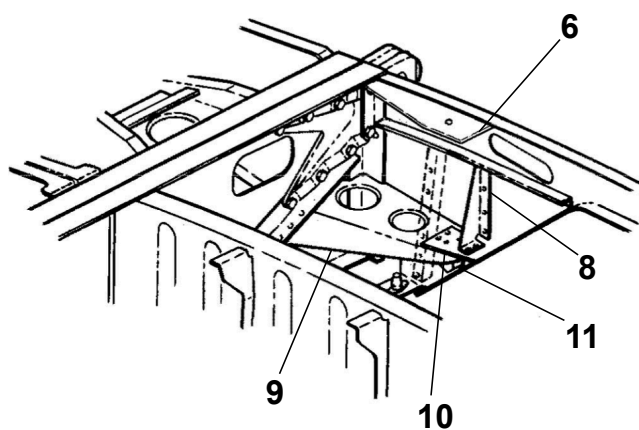
DETAIL C
