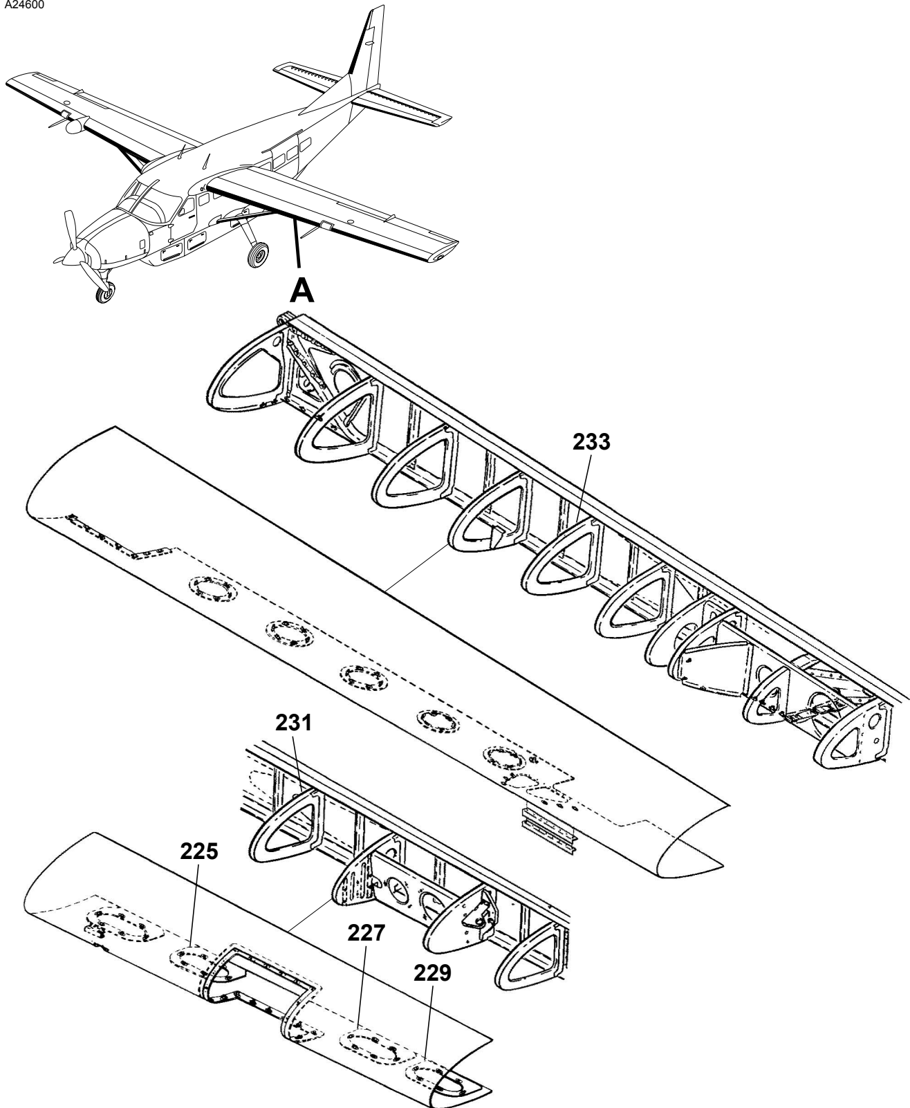
DETAIL A WING LEADING EDGE ASSEMBLIES Figure 01. (Sheet 4)
