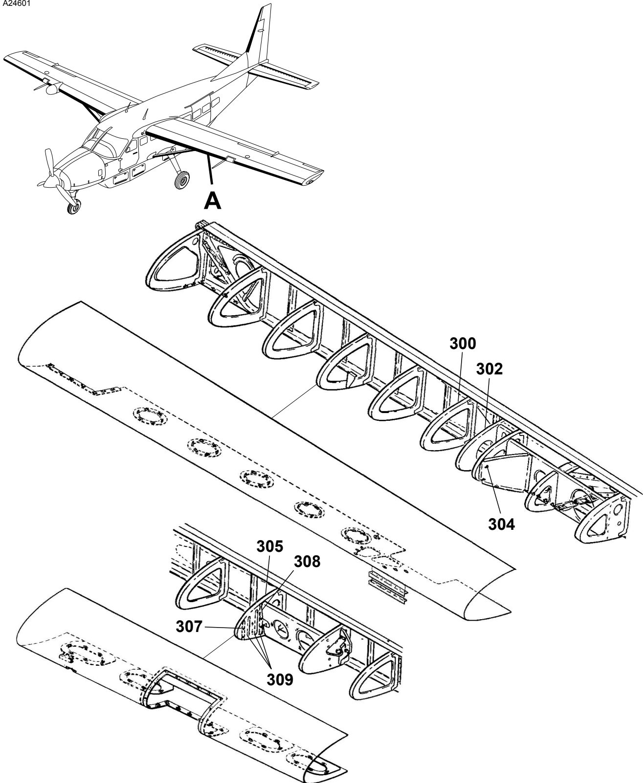
WING LEADING EDGE ASSEMBLIES Figure 01. (Sheet 5)
