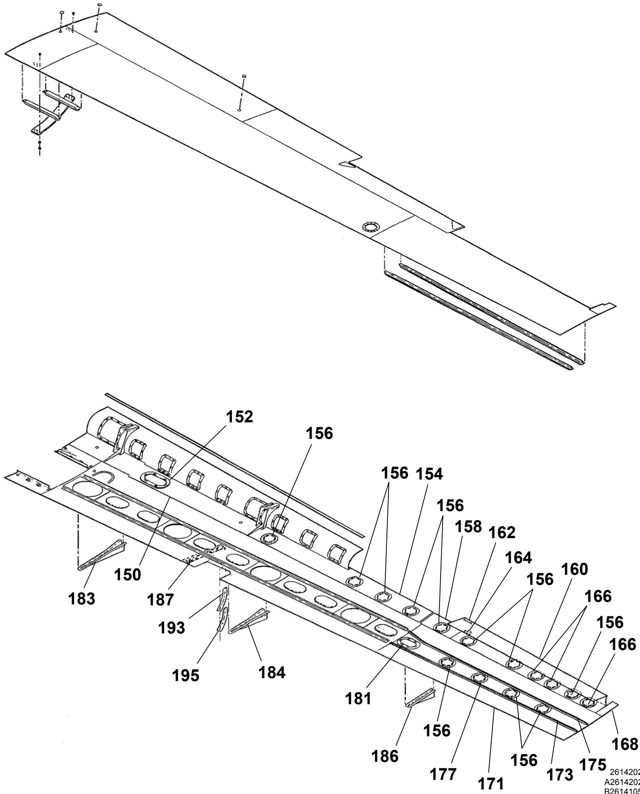
WING SKINS AND COMPONENTS Figure 01. (Sheet 3)
