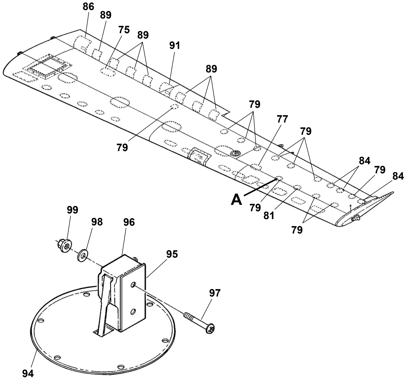
DETAIL A
