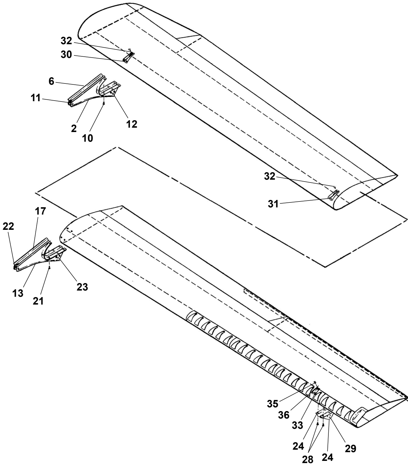
FLAP ASSEMBLY - STRUCTURE Figure 02. (Sheet 1)
