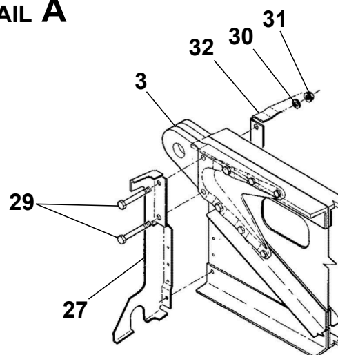
DETAIL B
