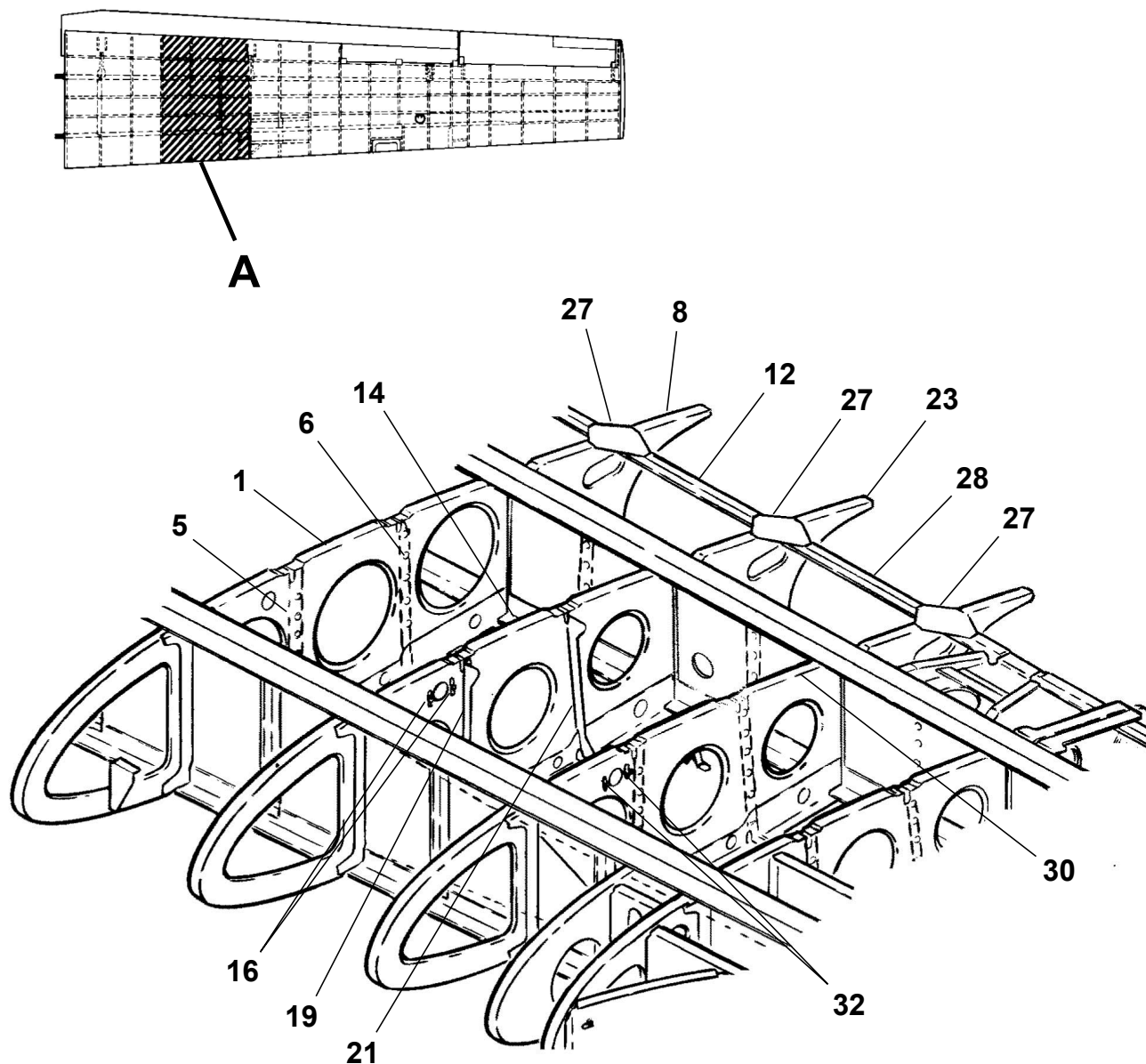
DETAIL A
