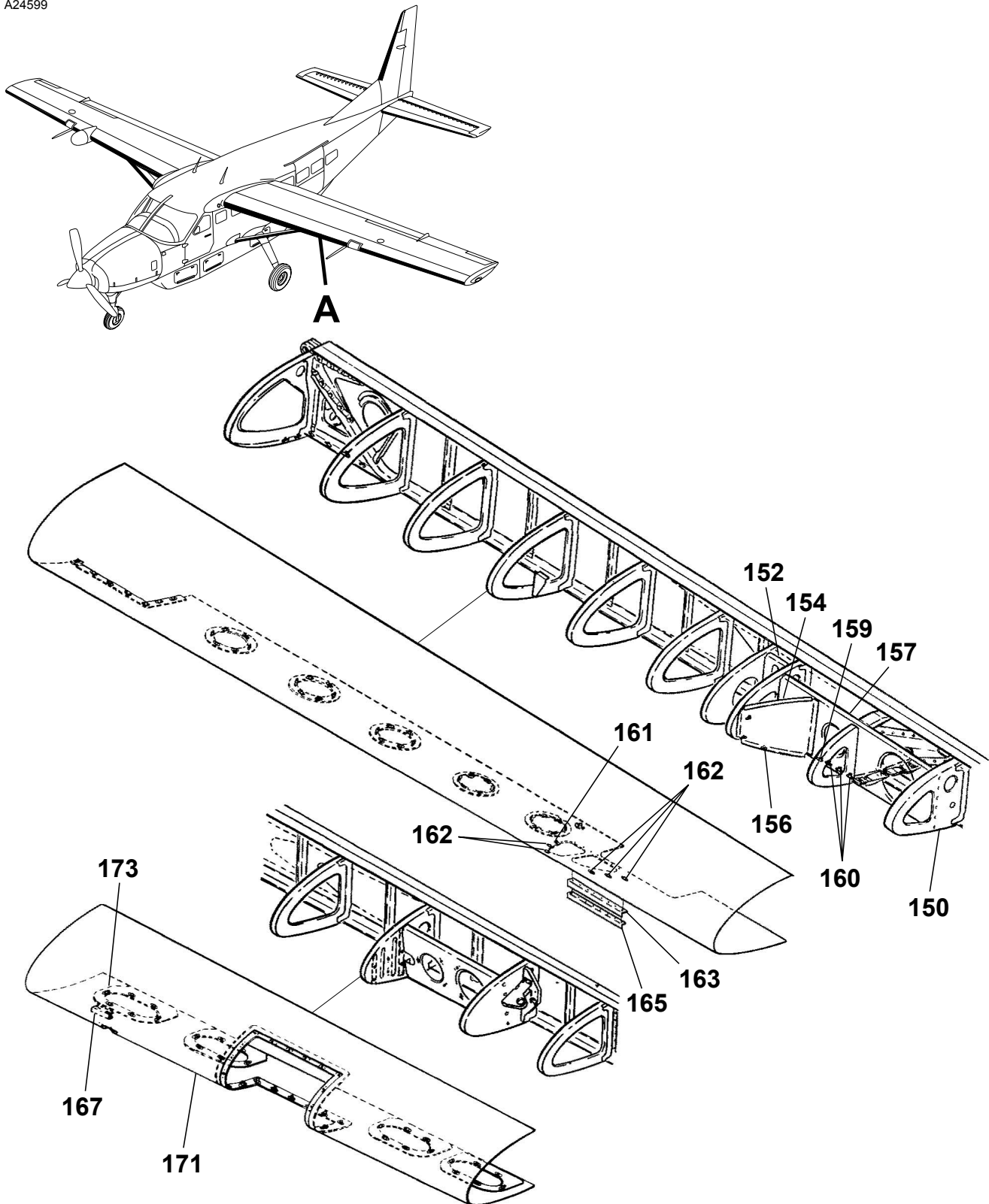
WING LEADING EDGE ASSEMBLIES Figure 01. (Sheet 3)
