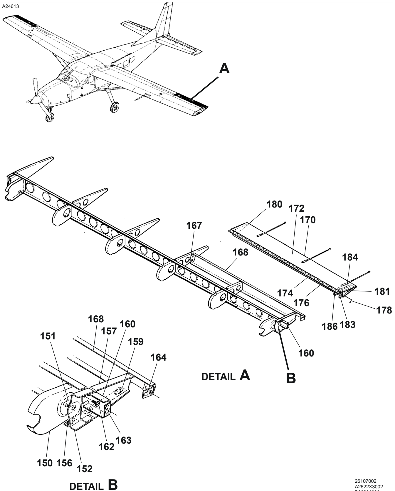
AILERON INSTALLATION Figure 01. (Sheet 3)
