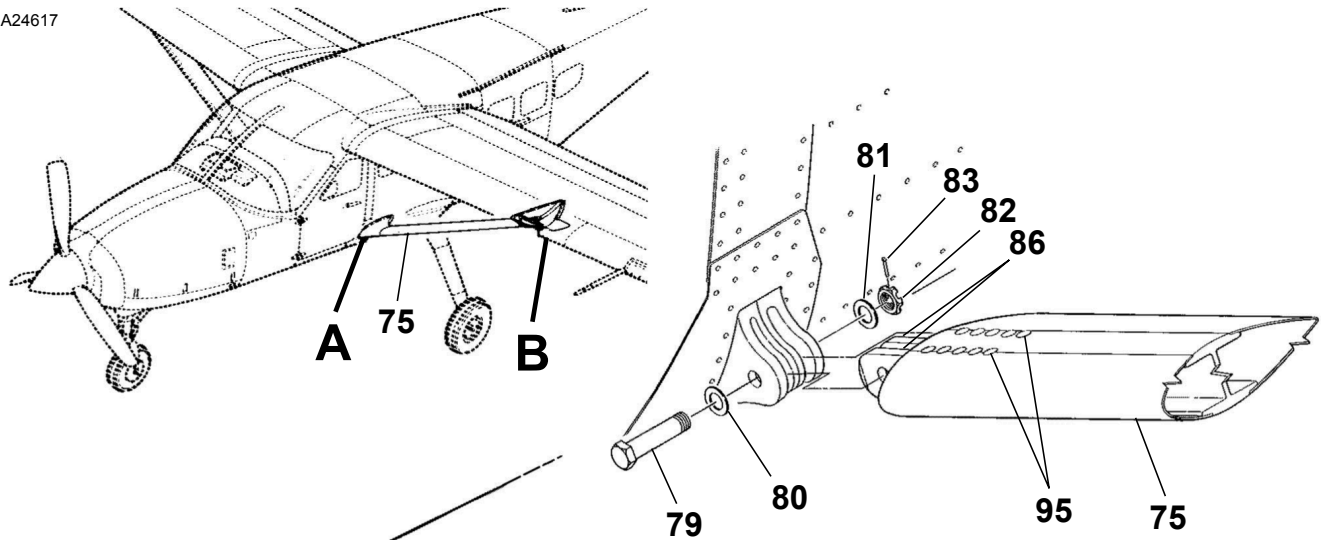
DETAIL A
