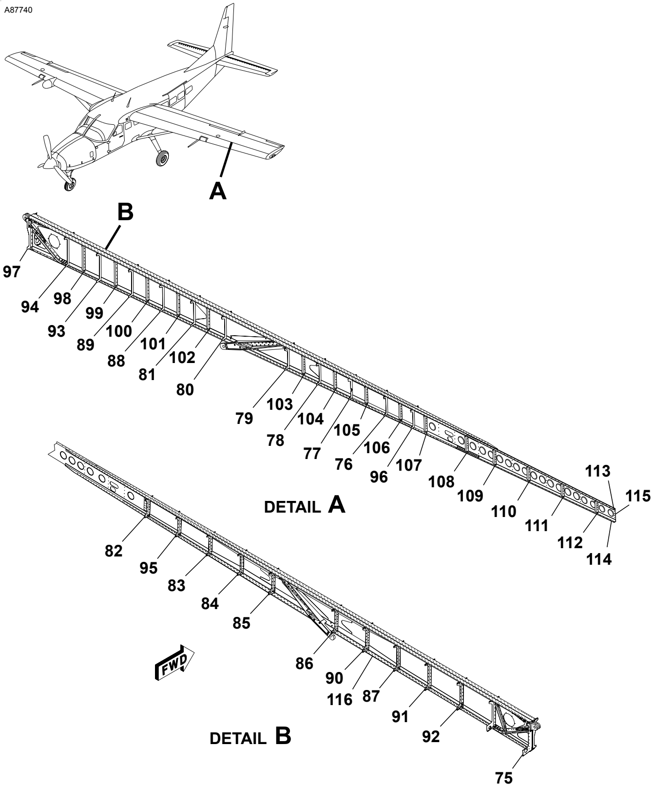
FRONT WING SPAR ASSEMBLIES - 208 & 208B Figure 03. (Sheet 2)
