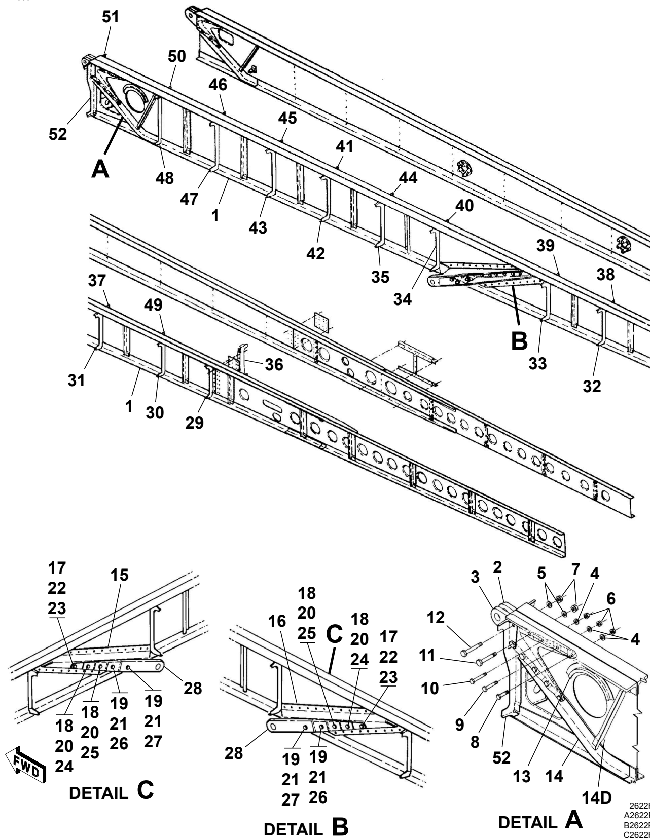
FRONT WING SPAR ASSEMBLIES - 208 Figure 01. (Sheet 1)
