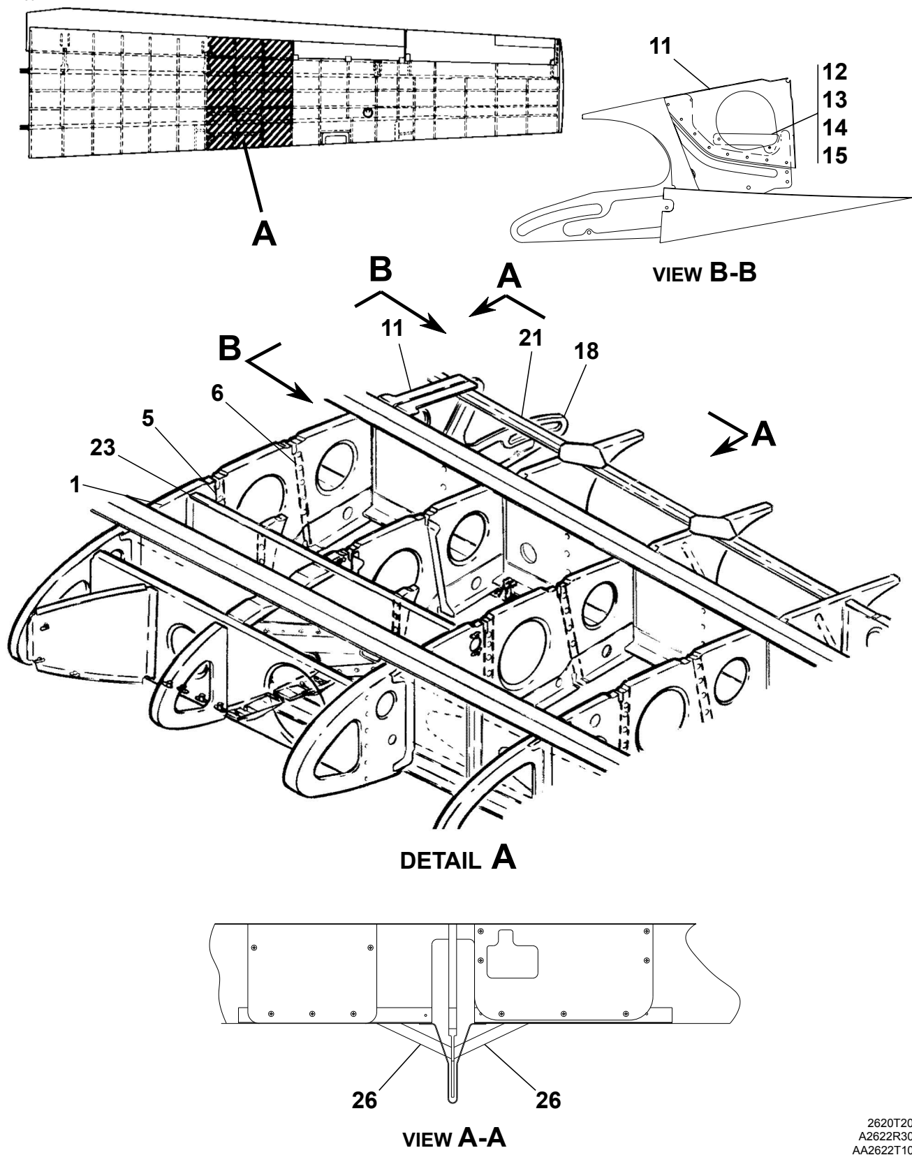
WING STRUCTURE COMPONENTS - FUEL BAY CENTER OUTBOARD Figure 03. (Sheet 1)
