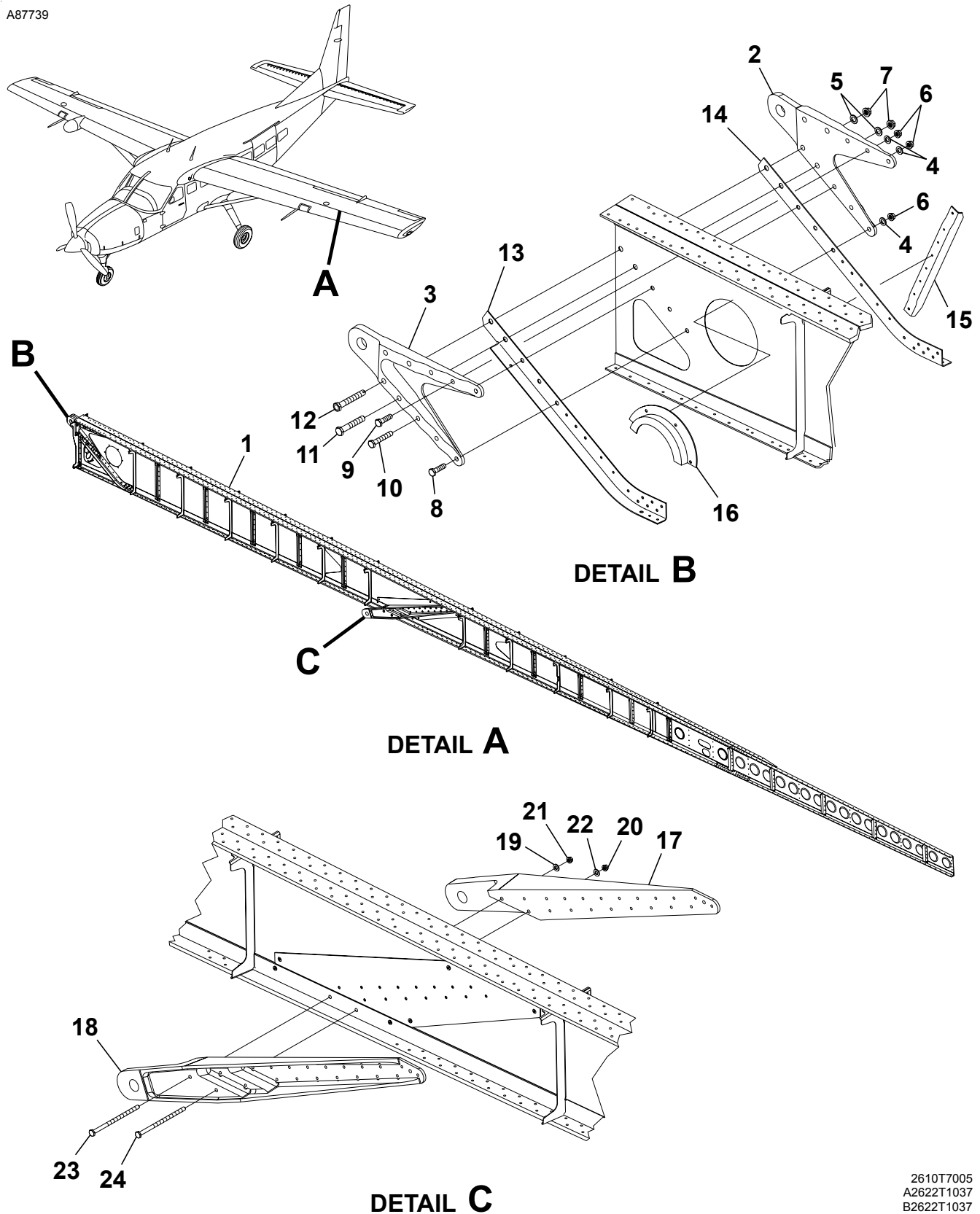
FRONT WING SPAR ASSEMBLIES - 208 & 208B Figure 03. (Sheet 1)
