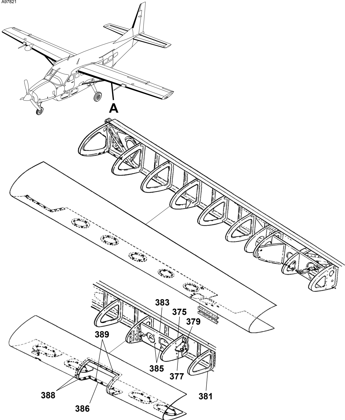
DETAIL A WING LEADING EDGE ASSEMBLIES Figure 01. (Sheet 6)
