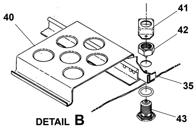
WING STRUCTURE COMPONENTS - FUEL BAY OUTBOARD Figure 04. (Sheet 1)
