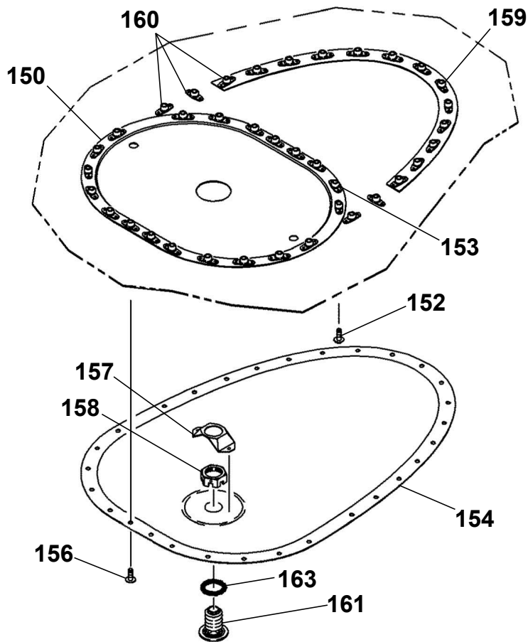
ACCESS PANELS - WING Figure 01. (Sheet 3)
